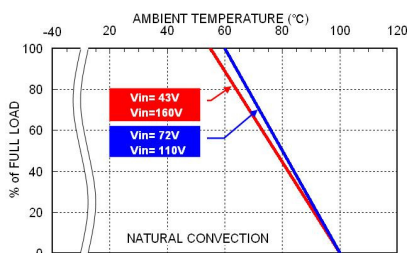
WAF300-110S With 3U Heat-sink Derating Curve
