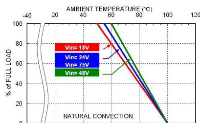
WAF300-48S With 3U Heat-sink Derating Curve
