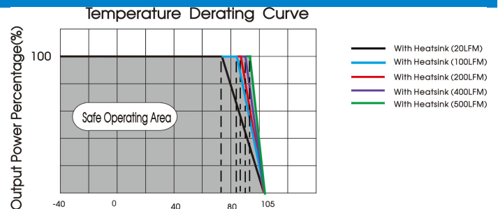
URF1D05QB-50WHR3 temperature derating curve (Vin=110V)
