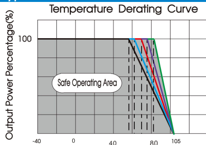
URF1D05QB-50WR3 temperature derating curve (Vin=110V)
