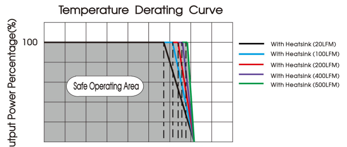
URF1D12QB-50WHR3 temperature derating curve (Vin=110V)
