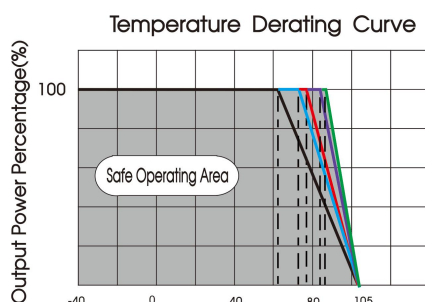
URF1D12QB-50WR3 temperature derating curve (Vin=110V)
