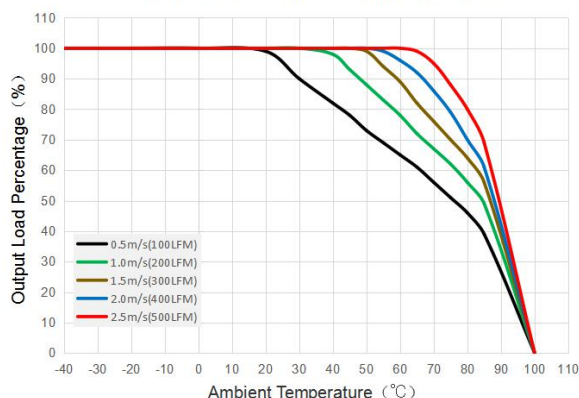
URF1D48HB-250WR3A7 Thermal Curves
