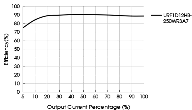
Efficiency Vs Output Load (Vin=110V)
