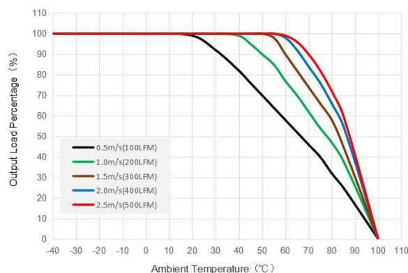
URF1D54HB-250WR3A7 Thermal Curves
