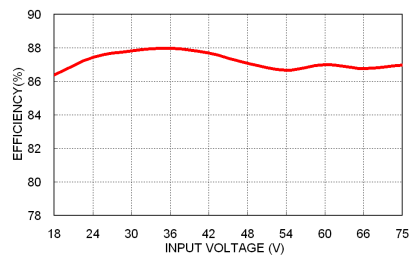
URED20-48S05W Efficiency vs. Input Voltage
