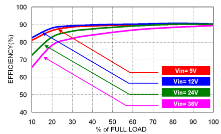
RCD15-24S05W Efficiency vs. Output Load
