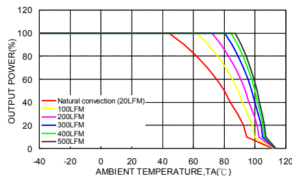
HAE150-48S05 Derating Curve With 0.24" Height Heat-sink
