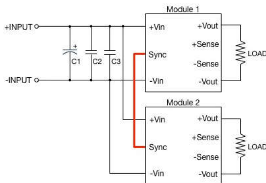
Synchronous Circuits
