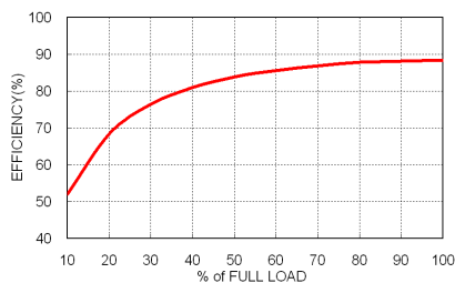
FED30-48S05W Efficiency vs. Output Load
