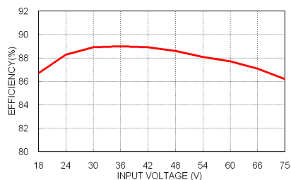
FED30-48S05W Efficiency vs. Input Voltage
