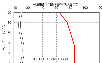
FED30-48S05W Derating Curve With Heat-sink
